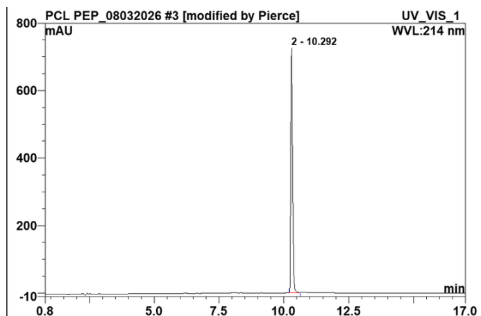
HPLC Chromatogram (Retention Time: 10.29 min)
